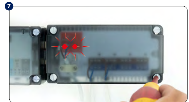
Make sure that all the wires are properly connected, mount top cover and power up the wiring centre - "Power" and "Connection" red LED diodes will light up indicating the correct connection with the KL08RF wiring centre.
